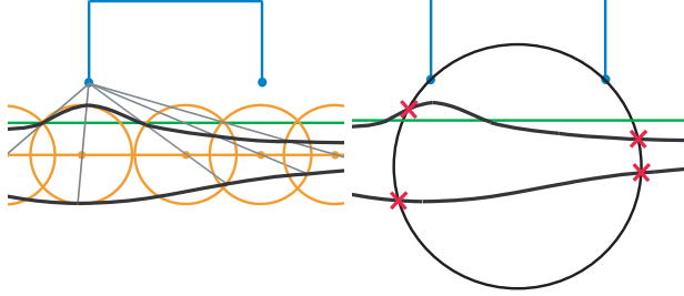
Fig. 3. Left: The picture shows the Constraint C_2 for the ball, some of the circles according to constraint C_5 , some of the lines according to C_4 , and the resulting two lines for C_6 (bold black lines). Right: Constraints according to C_7 : The position of the robot is one of the four intersection points between the periphery circle ( C_1 ) and the lines according to C_6 .
